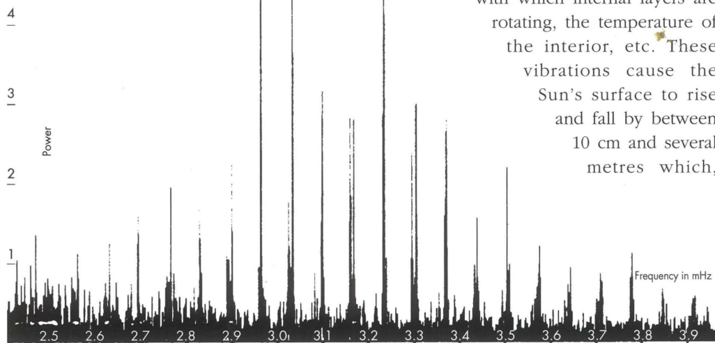
Diagram of the Sun's 5 minute vibrations as measured at the South Pole.
