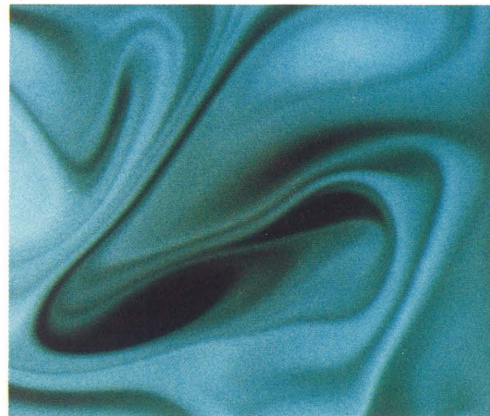
Numerical simulation of turbulent flow displayed on a computer screen.
